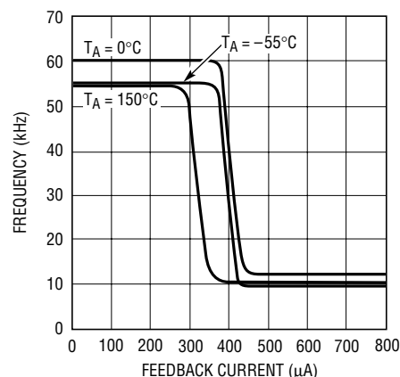
Short-Circuit Frequency Shift-Down vs Feedback Current
