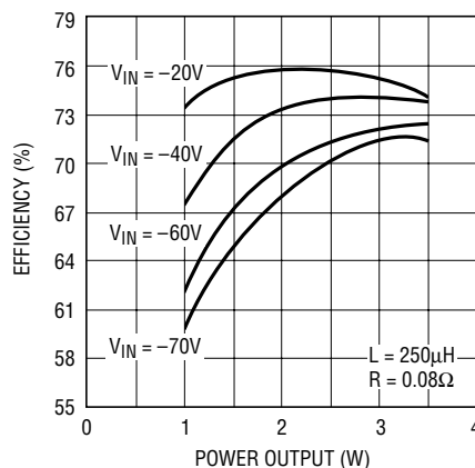
Telecom 5V Supply Efficiency
