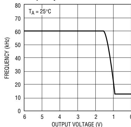
Telecom 5V Supply Short-Circuit Frequency Shift-Down
